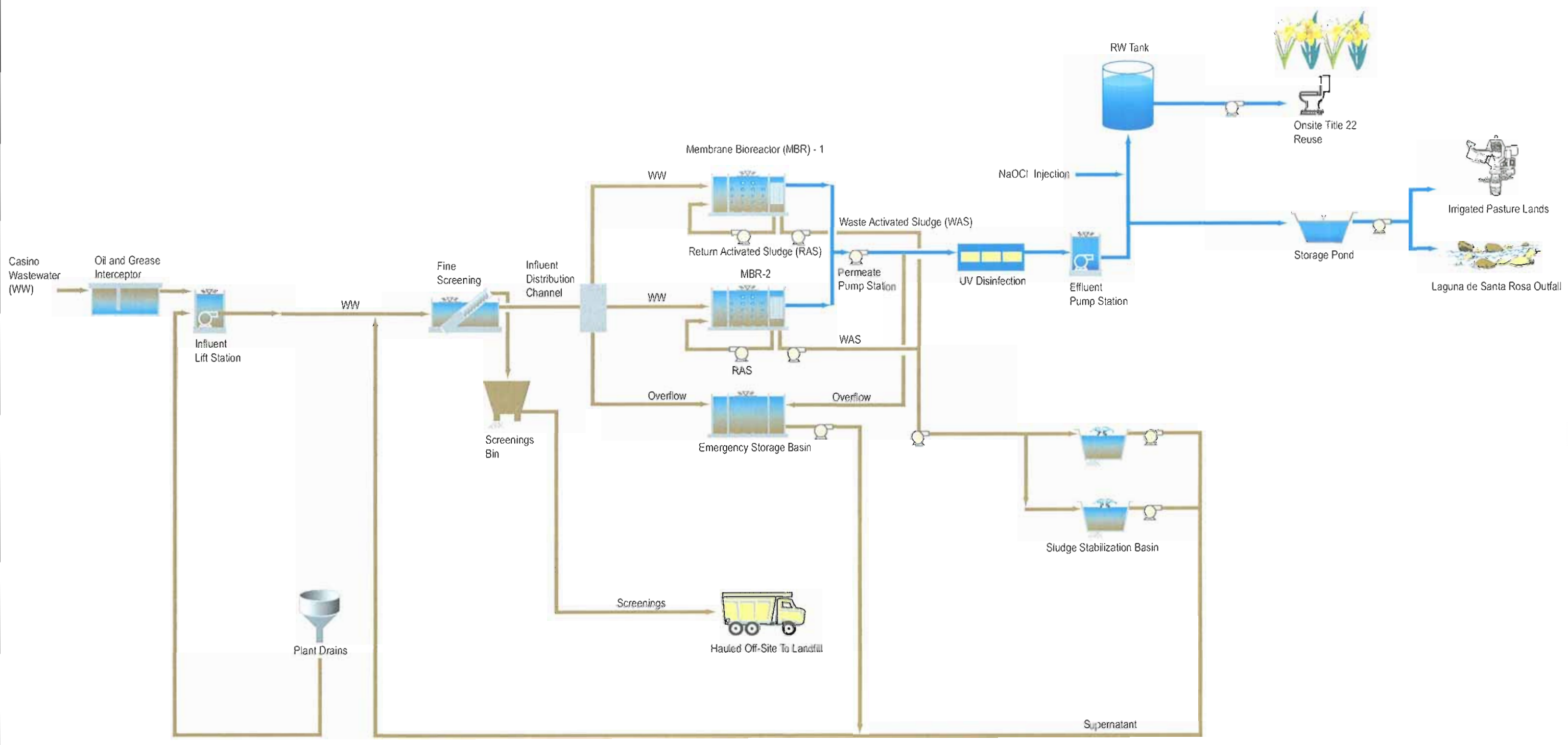
FIGURE 2-3 STATION CASINOS GRATON RANCHERIA HOTEL AND CASINO PROJECT WASTEWATER TREATMENT PROCESS FLOW DIAGRAM
