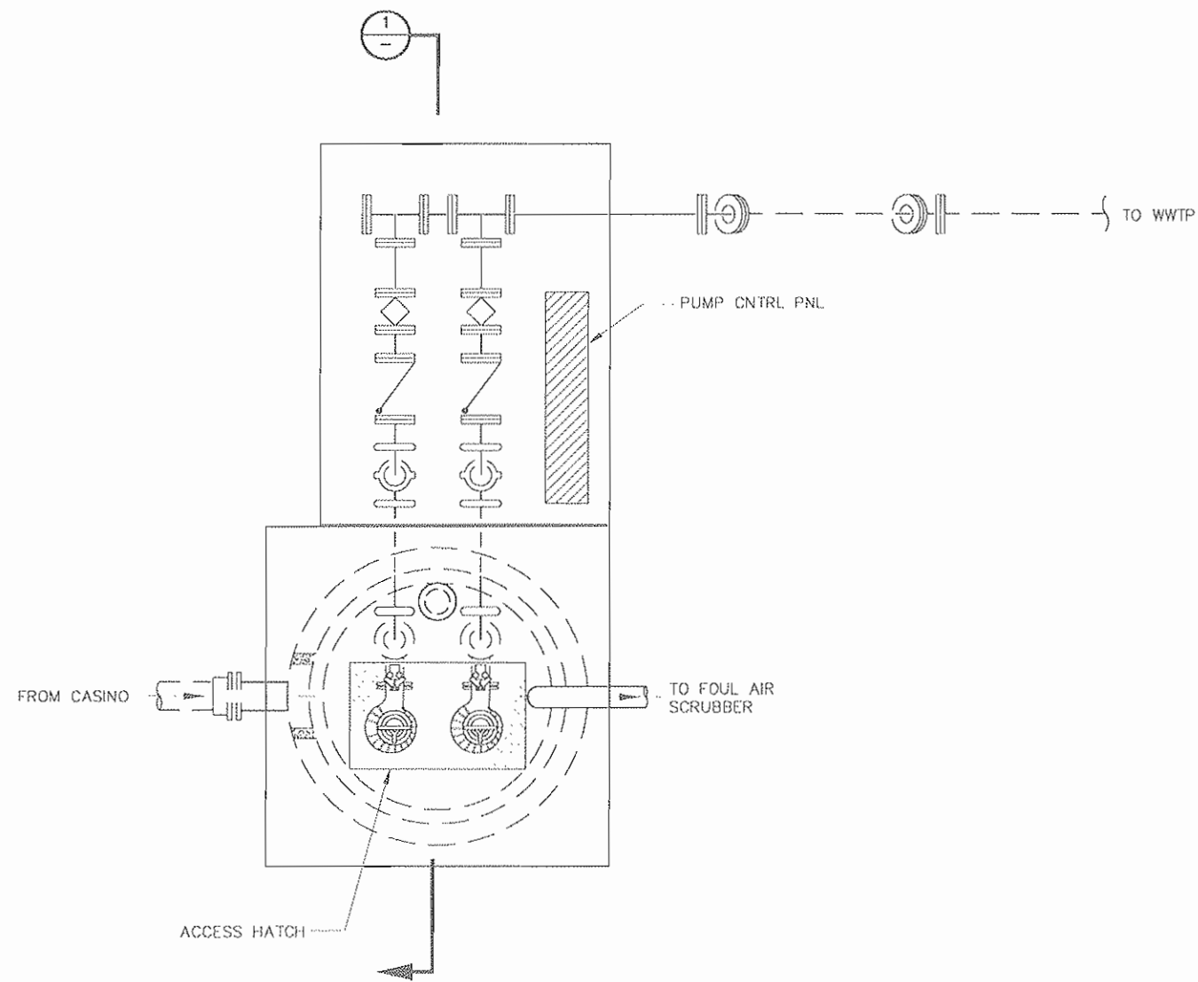
TYPICAL LIFT STATION PLAN SCALE: 1/4" = 1'-0"
