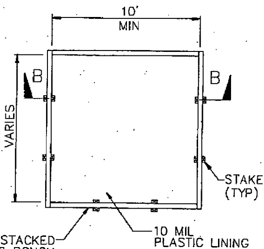
PLAN NOT TO SCALE TYPE "ABOVE GRADE"
