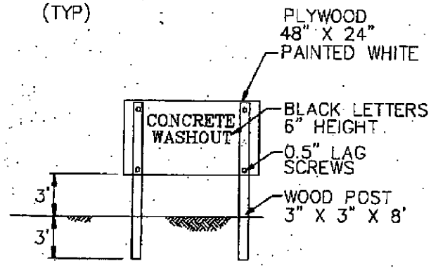
CONCRETE WASHOUT SIGN DETAIL (OR EQUIVALENT)
